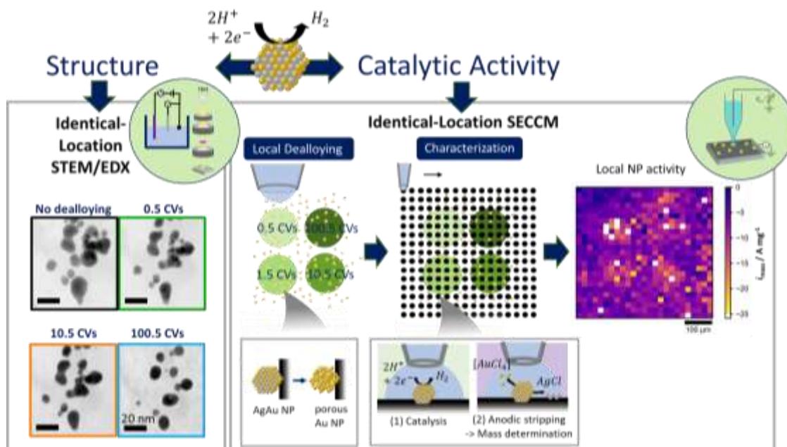
Figure 1. Schematic measurement concept for dealloying of Ag x Au y NPs by successive cycling in acid. Left: Identical-location STEM images of NPs at four different dealloying states (numbers of cycles). Right: Local dealloying with big SECCM tip, followed by catalytic activity measurements on many locations with a small tip for statistical analysis
