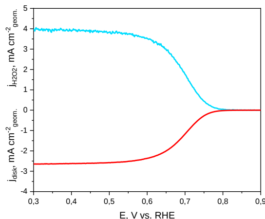
Figure 1. The RRDE polarization curves of NCC heating-cooling samples in \text{O}_2 -saturated 0.1 M KOH, produced through rapid heating and cooling stages during MW heating.
