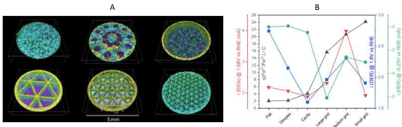
Figure 1. (A) Images taken by NCOP (B) Activities of the manufactured electrodes towards the Fe 2+/3+ redox, oxygen evolution, hydrogen evolution, and ethanol oxidation reactions
