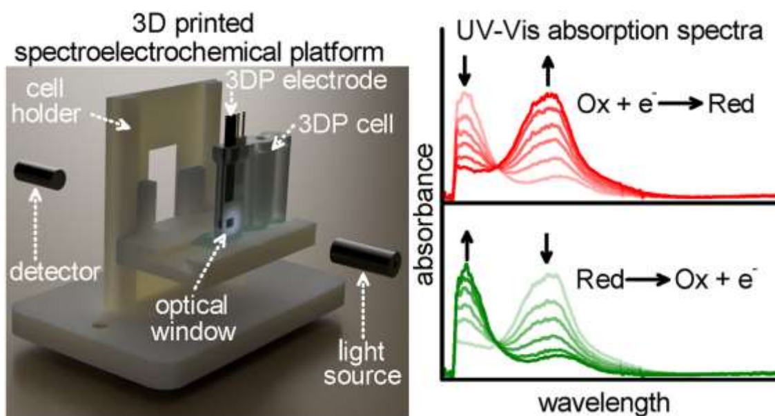
Figure 1. 3D printed spectroelectrochemical platform
