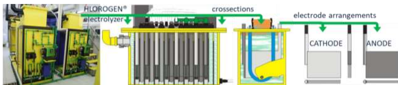
Figure 1. HLOROGEN® electrolyzers: a) complete plant – Novi Sad water supply, b) crosssections – side views with electrode compartments and cooling system, c) electrode arrangement with 3 cathodes and 2 anodes per electrode compartment
