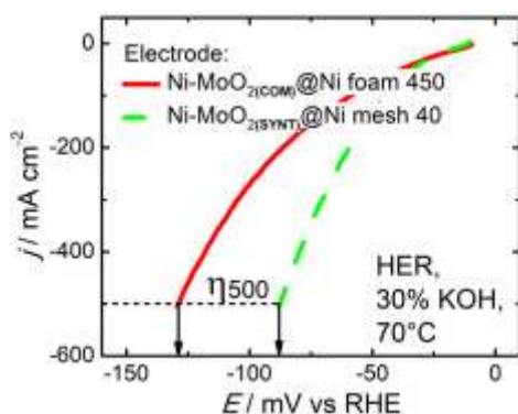
Figure 1. HER polarization curves recorded at porous electrodes coated with composite coatings based on commercial (COM) and synthesized (SYNT) \text{MoO}_2
