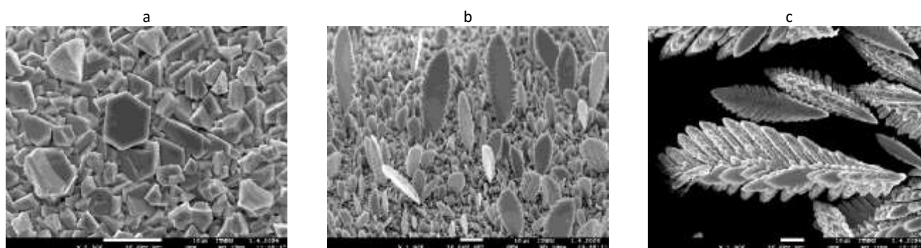
Figure 1. Morphology of Zn disperse forms electrodeposited at overpotentials of: a) 160 mV, b) 220 mV, and c) 280 mV. The amount of electricity: 3.0 \text{ mAh cm}^{-2} .
