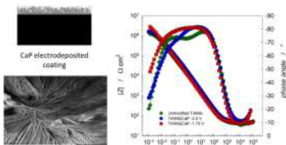
Figure 1. The SEM image of electrodeposited CaP coating presented with Bode plots of the unmodified and the CaP-coated TiAlNb alloy recorded in Hank's solution at open circuit potential.
