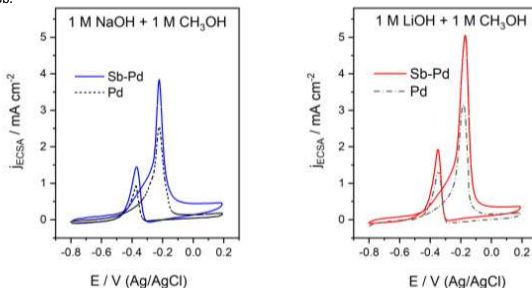
Figure 1. CVs for the electrochemical oxidation of 1 M \text{CH}_3\text{OH} at Pd and Sb–Pd in 1 M NaOH and 1 M LiOH at v = 0.05 \text{ Vs}^{-1} .
